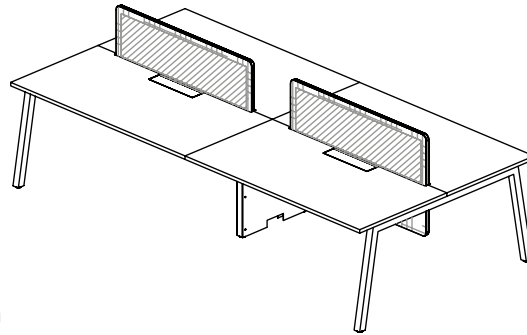
High Desk 2 Clusters Width 1500mm Depth 1500mm Height 1355mm
