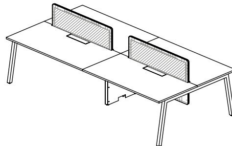
Low Desk 2 Clusters Width 1500mm Depth 11480mm Height 720mm
